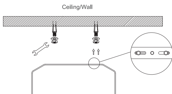
A : Install the setscrews
