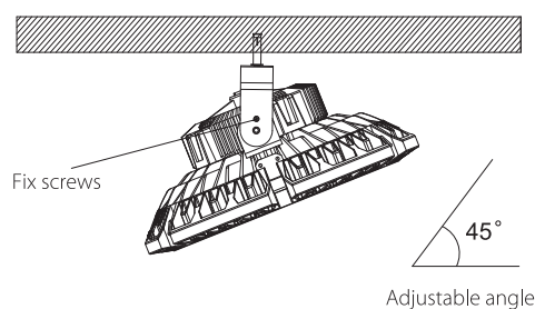
D: Adjust the lamp angle and clean it.
