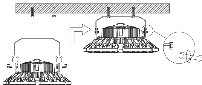
B: Put the lamp card into the setscrews and lock it tightly
